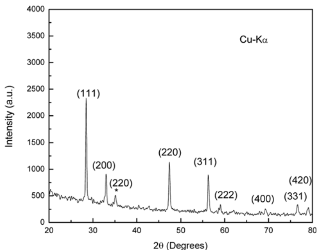
Fig. 2. XRD pattern of CSCMn powders after reduction in 3% \text{H}_2 - \text{N}_2 at 1,100^\circ\text{C} for 5 h (* standing for \text{CeO} (200)).
