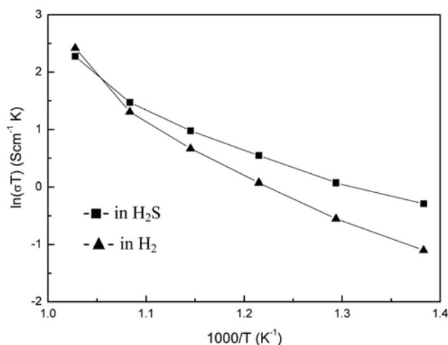
Fig. 6. Conductivities of CSCMn in 5% \text{H}_2\text{S}-\text{N}_2 and 3% \text{H}_2-\text{N}_2 at various temperatures.
